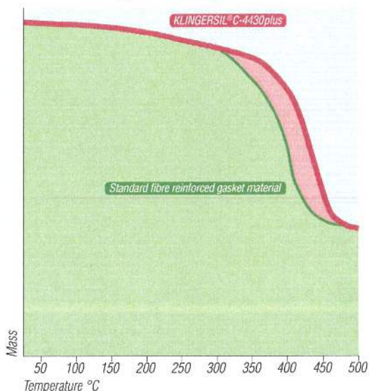
Thermogravimetric analysis
