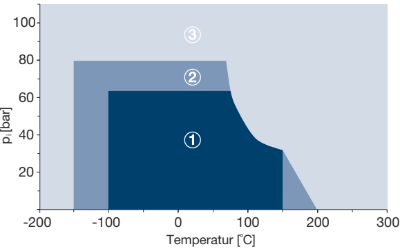
P-T Diagramm - Dicke 2,0 mm
