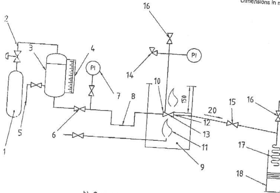
b) Compressed gas as pressure source
